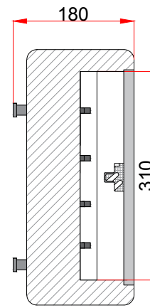
SIDE VIEW / SECTION
