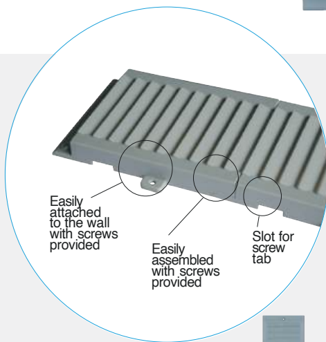
Top & base pack + 2 mid sections (single strip)
